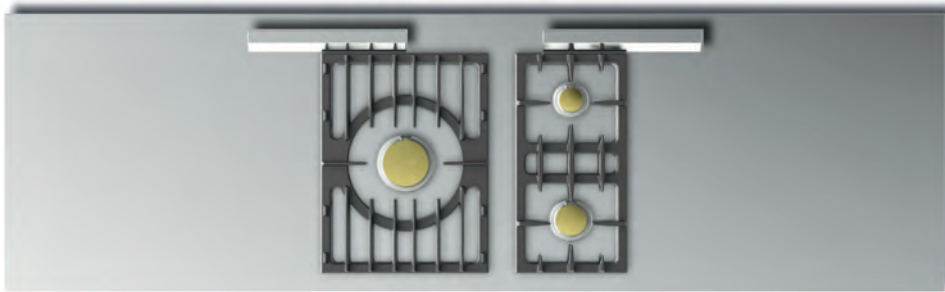
CLASSIC HOB 3 BURNERS (5kW BURNER UNDER SIMMER PLATE) 1 burner @ 5kW 1 burner @ 3kW 1 burner @ 1.5kW + 4 integrated hob options
